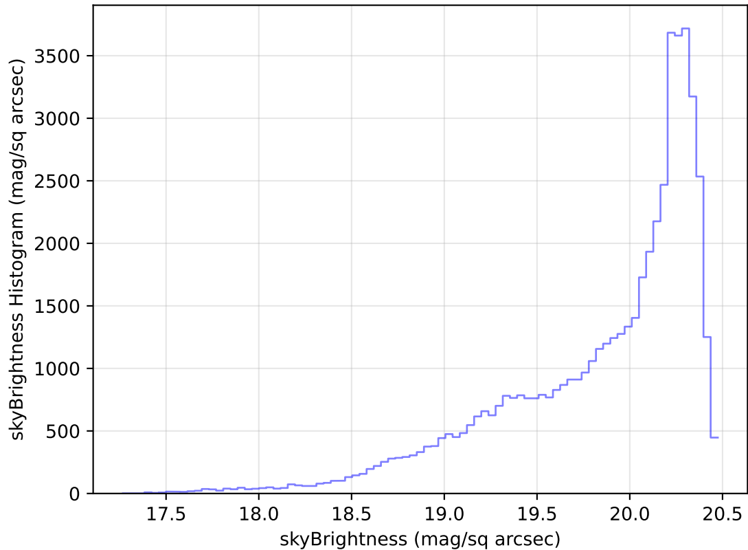
too_elab_heavy_r64_d2_griz_v3.4_10yrs Yr 1 i band: skyBrightness Histogram
