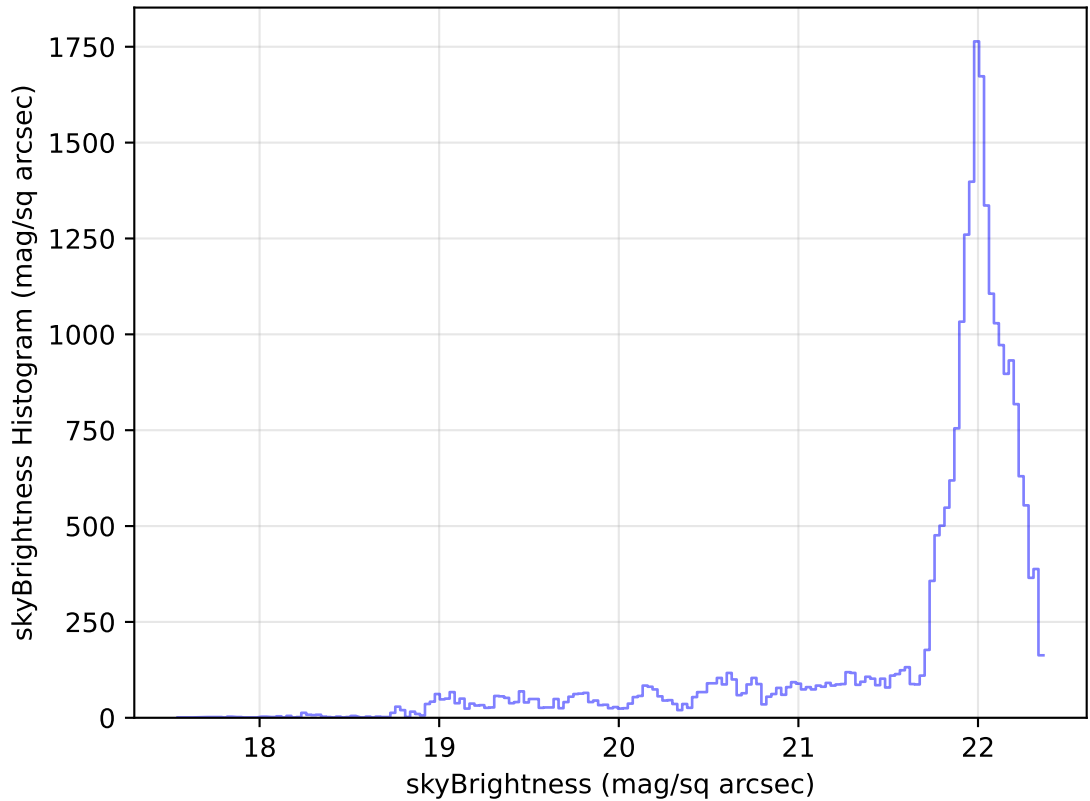
too_elab_heavy_r64_d2_griz_v3.4_10yrs Yr 1 g band: skyBrightness Histogram
