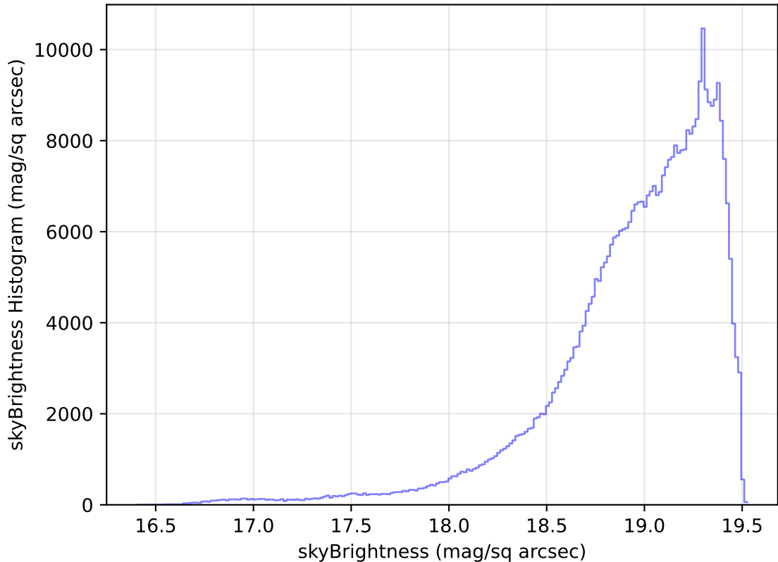
too_elab_heavy_r64_d2_griz_v3.4_10yrs WFD z band: skyBrightness Histogram
