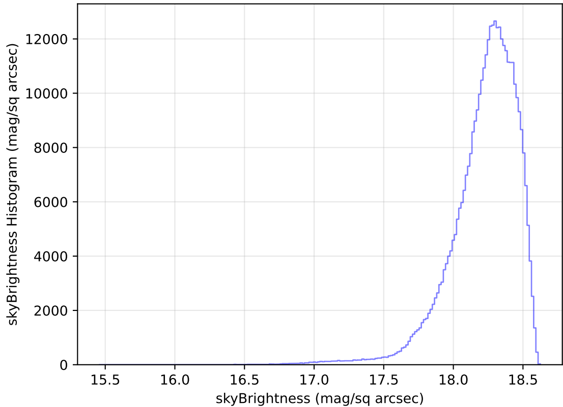
too_elab_heavy_r64_d2_griz_v3.4_10yrs WFD y band: skyBrightness Histogram
