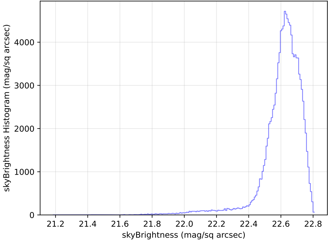
too_elab_heavy_r64_d2_griz_v3.4_10yrs WFD u band: skyBrightness Histogram
