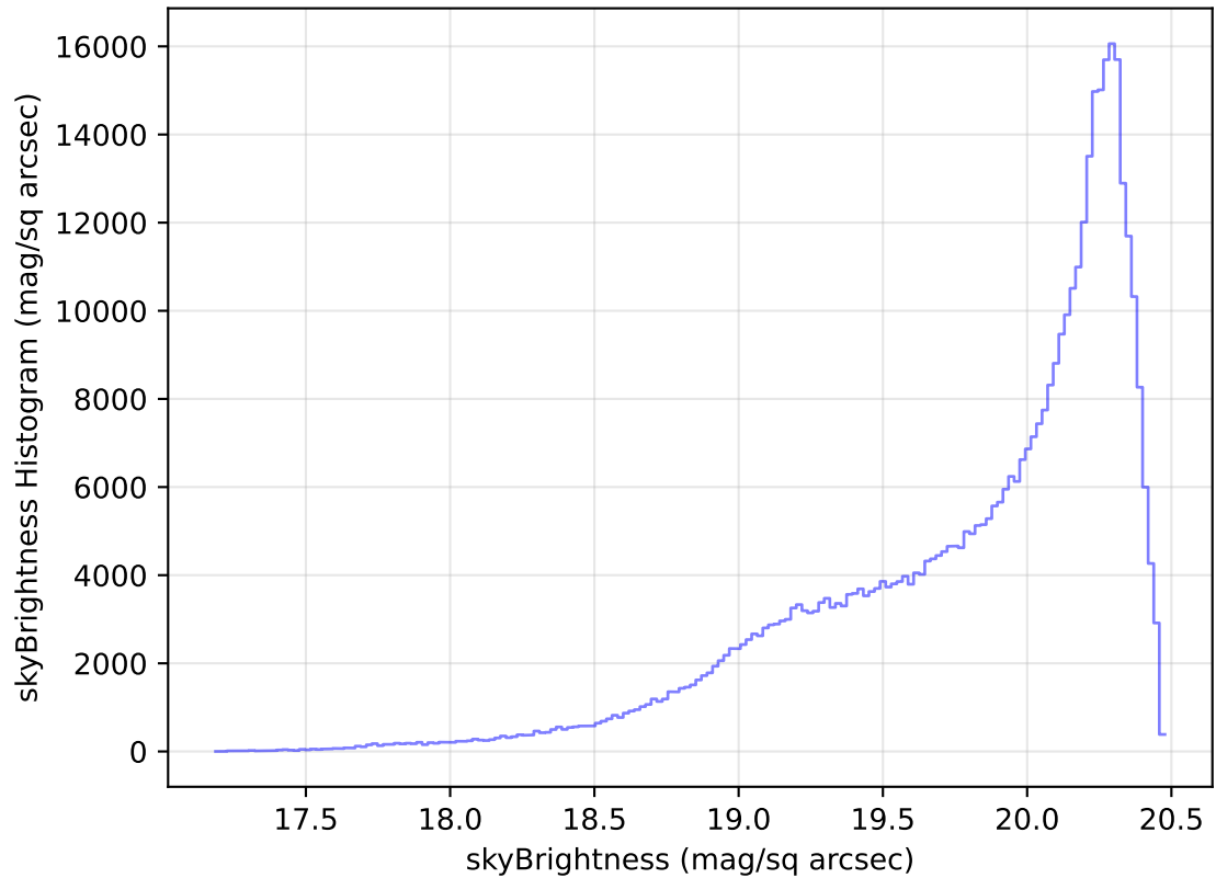
too_elab_heavy_r64_d2_griz_v3.4_10yrs WFD i band: skyBrightness Histogram
