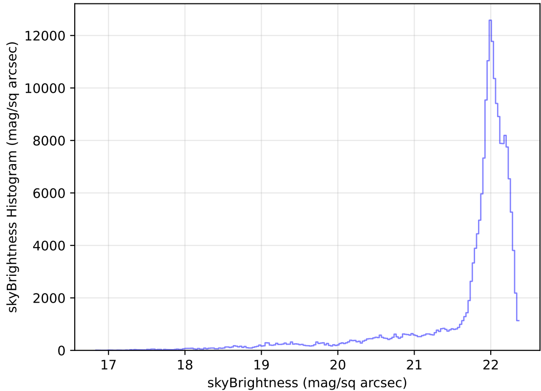
too_elab_heavy_r64_d2_griz_v3.4_10yrs WFD g band: skyBrightness Histogram
