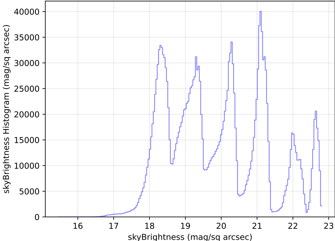
too_elab_heavy_r64_d2_griz_v3.4_10yrs WFD all bands: skyBrightness Histogram
