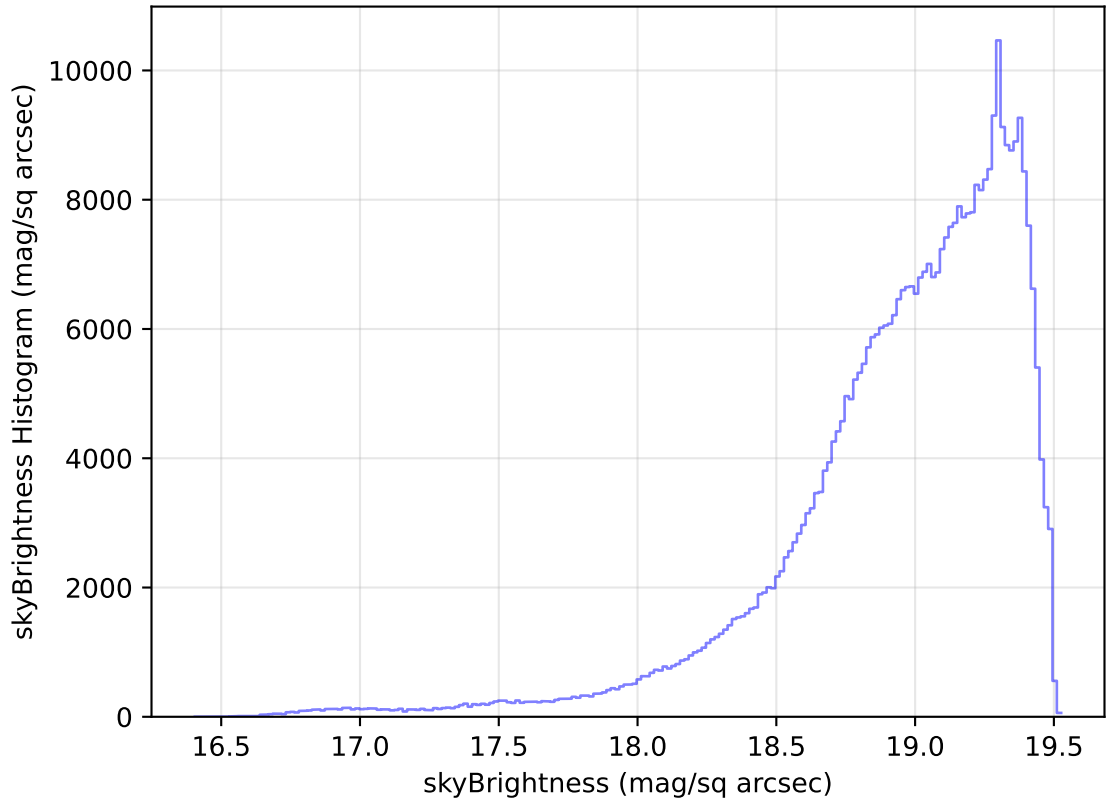
too_elab_heavy_r64_d2_griz_v3.4_10yrs All sky z band: skyBrightness Histogram
