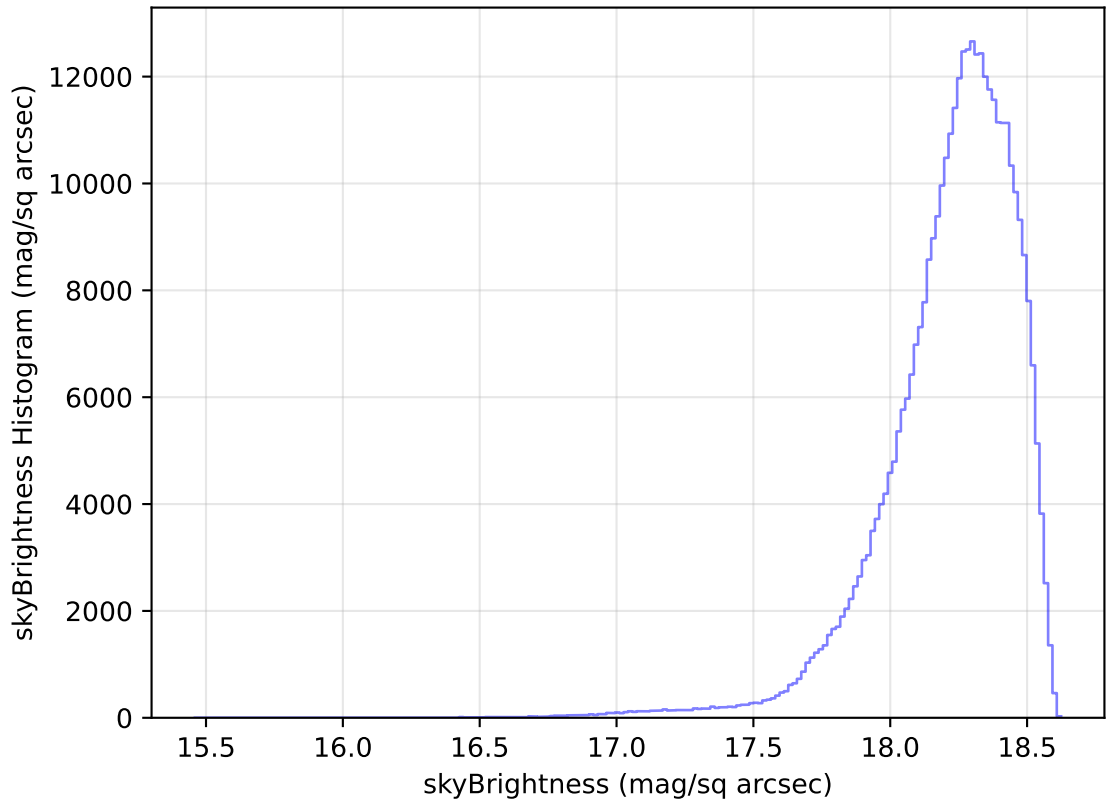
too_elab_heavy_r64_d2_griz_v3.4_10yrs All sky y band: skyBrightness Histogram
