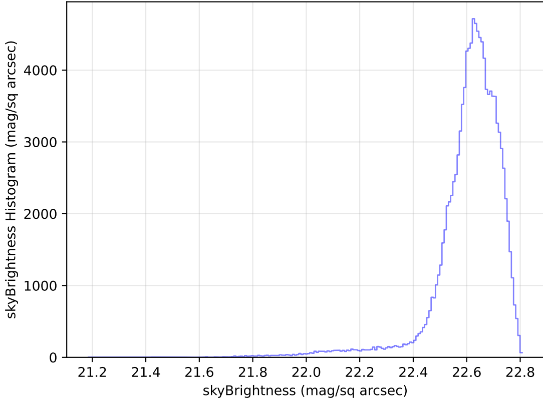
too_elab_heavy_r64_d2_griz_v3.4_10yrs All sky u band: skyBrightness Histogram
