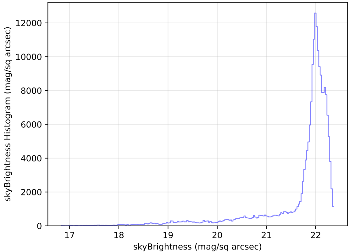
too_elab_heavy_r64_d2_griz_v3.4_10yrs All sky g band: skyBrightness Histogram
