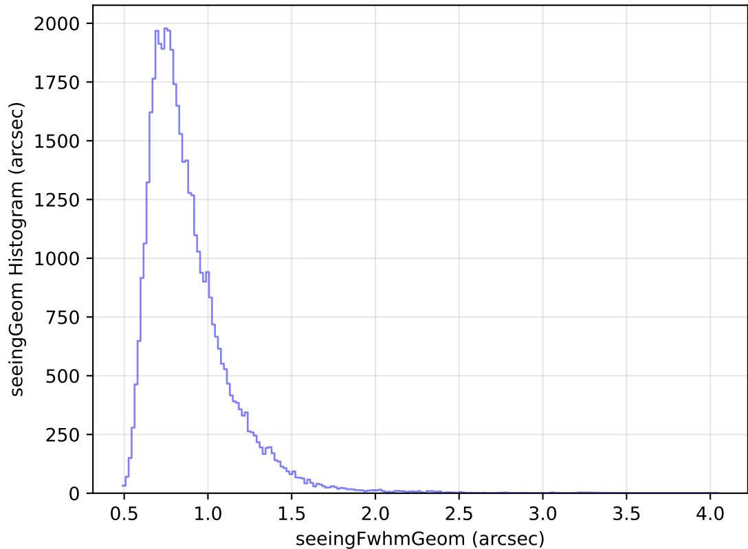
too_elab_heavy_r64_d2_griz_v3.4_10yrs Yr 1 z band: seeingGeom Histogram
