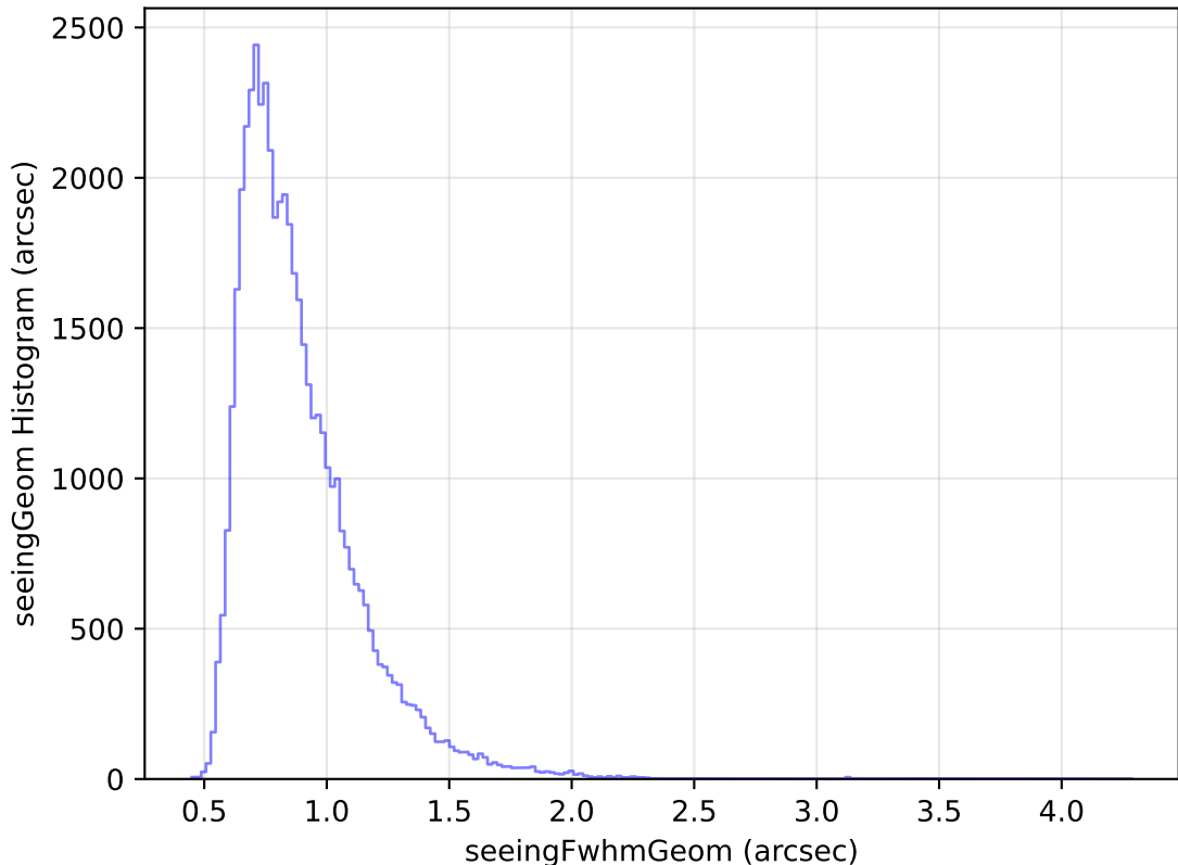
too_elab_heavy_r64_d2_griz_v3.4_10yrs Yr 1 r band: seeingGeom Histogram
