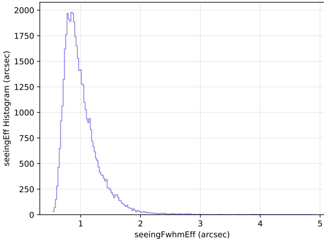
too_elab_heavy_r64_d2_griz_v3.4_10yrs Yr 1 z band: seeingEff Histogram
