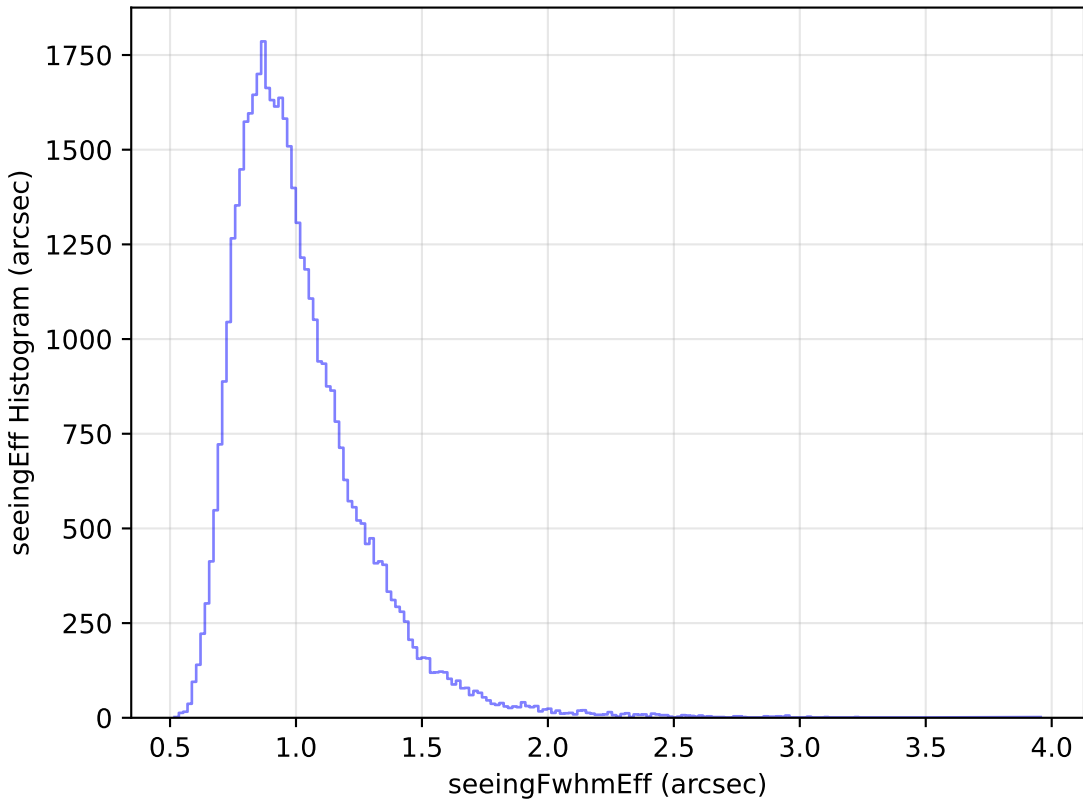
too_elab_heavy_r64_d2_griz_v3.4_10yrs Yr 1 y band: seeingEff Histogram
