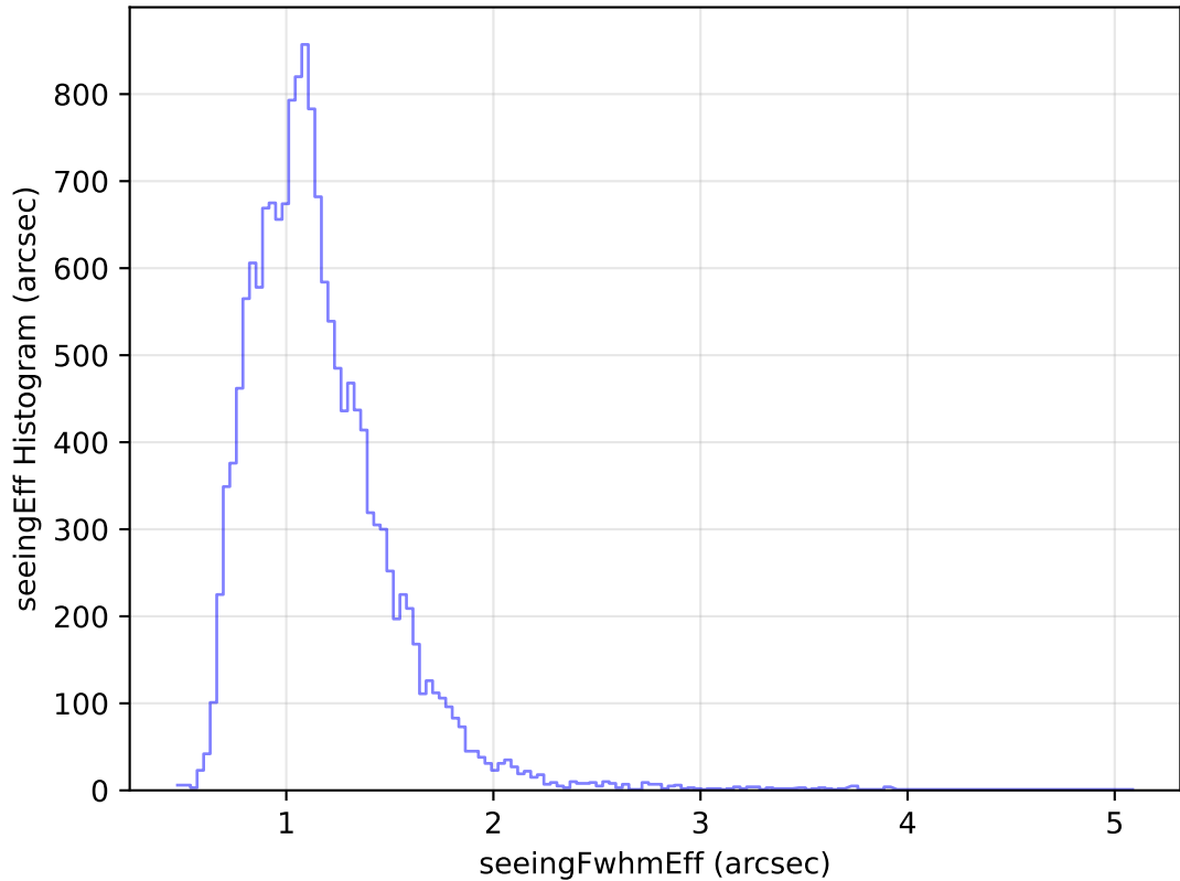
too_elab_heavy_r64_d2_griz_v3.4_10yrs Yr 1 u band: seeingEff Histogram
