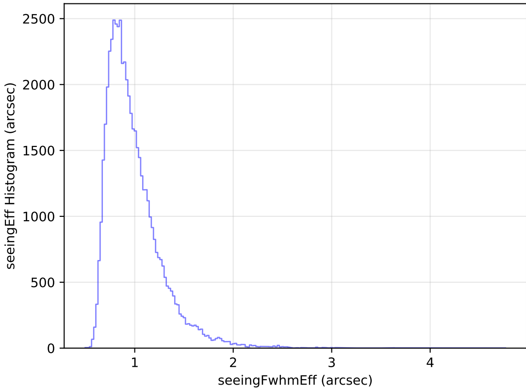
too_elab_heavy_r64_d2_griz_v3.4_10yrs Yr 1 i band: seeingEff Histogram
