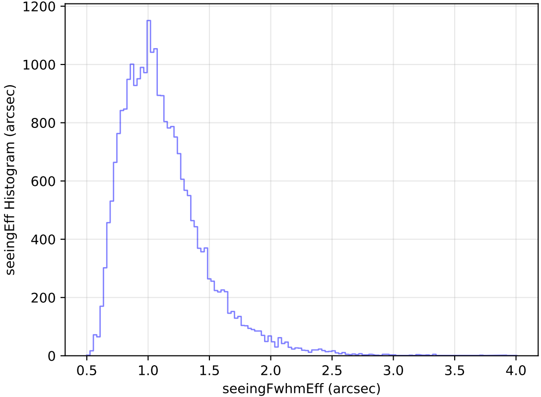
too_elab_heavy_r64_d2_griz_v3.4_10yrs Yr 1 g band: seeingEff Histogram
