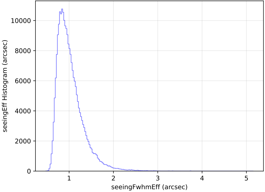
too_elab_heavy_r64_d2_griz_v3.4_10yrs Yr 1 all bands: seeingEff Histogram
