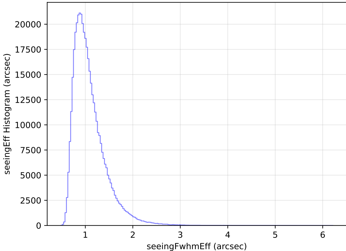
too_elab_heavy_r64_d2_griz_v3.4_10yrs WFD z band: seeingEff Histogram
