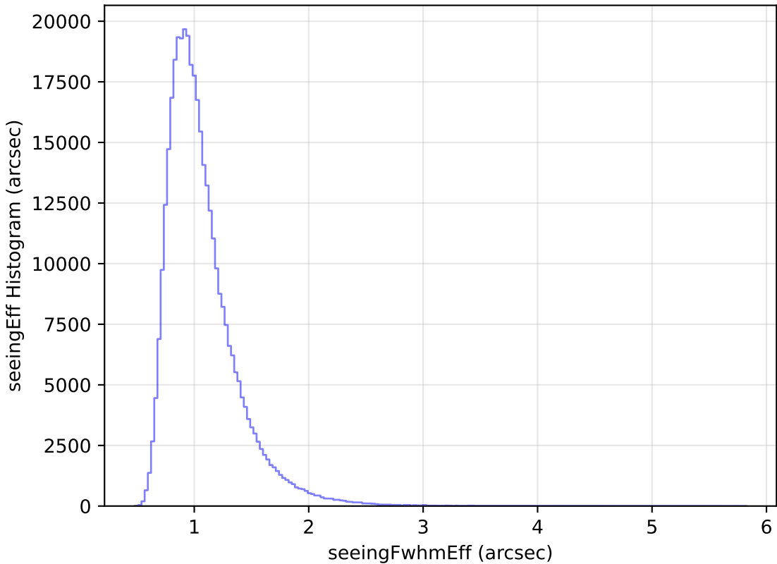
too_elab_heavy_r64_d2_griz_v3.4_10yrs WFD y band: seeingEff Histogram
