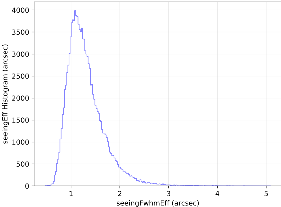
too_elab_heavy_r64_d2_griz_v3.4_10yrs WFD u band: seeingEff Histogram
