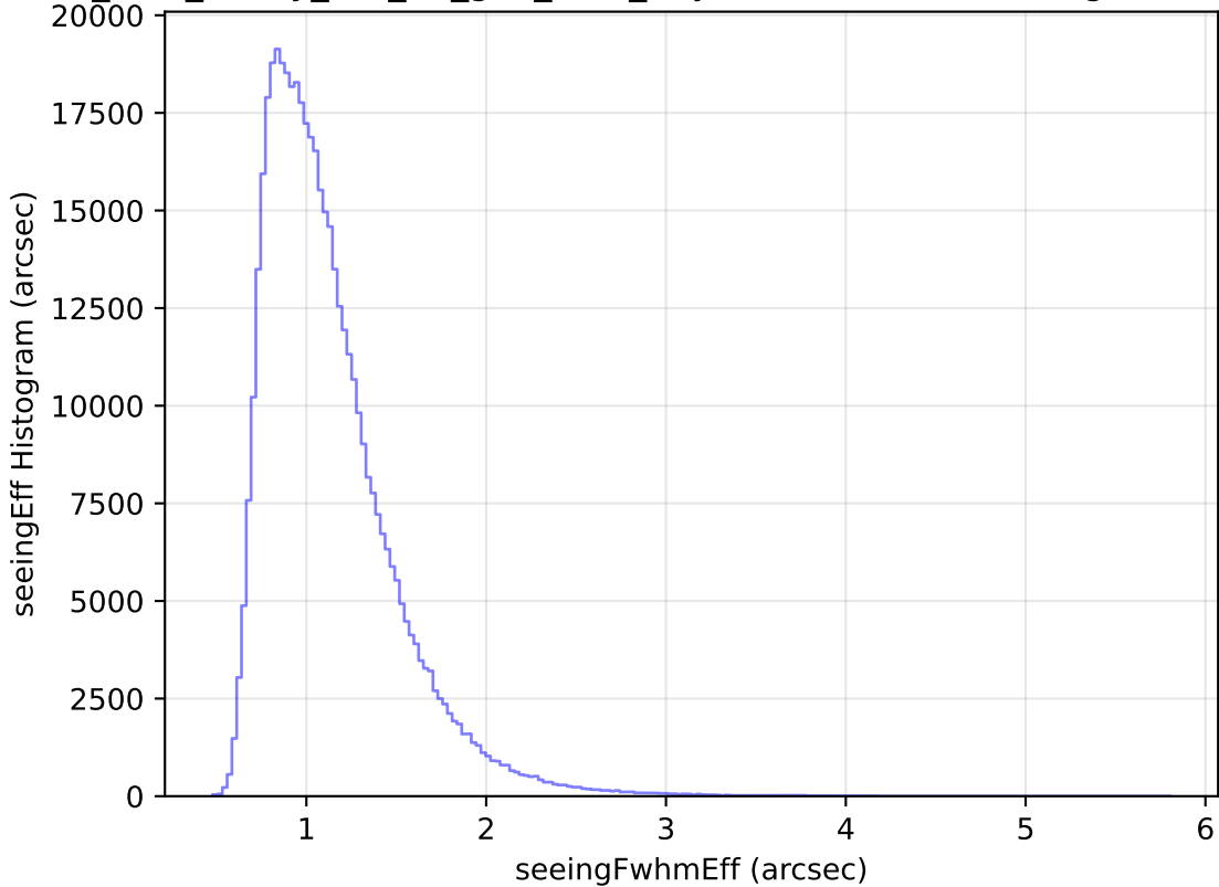
too_elab_heavy_r64_d2_griz_v3.4_10yrs WFD r band: seeingEff Histogram
