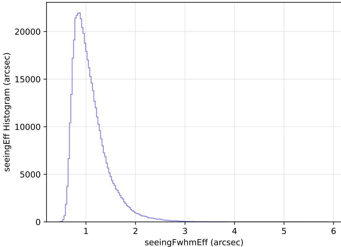
too_elab_heavy_r64_d2_griz_v3.4_10yrs WFD i band: seeingEff Histogram
