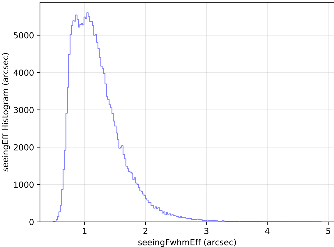
too_elab_heavy_r64_d2_griz_v3.4_10yrs WFD g band: seeingEff Histogram
