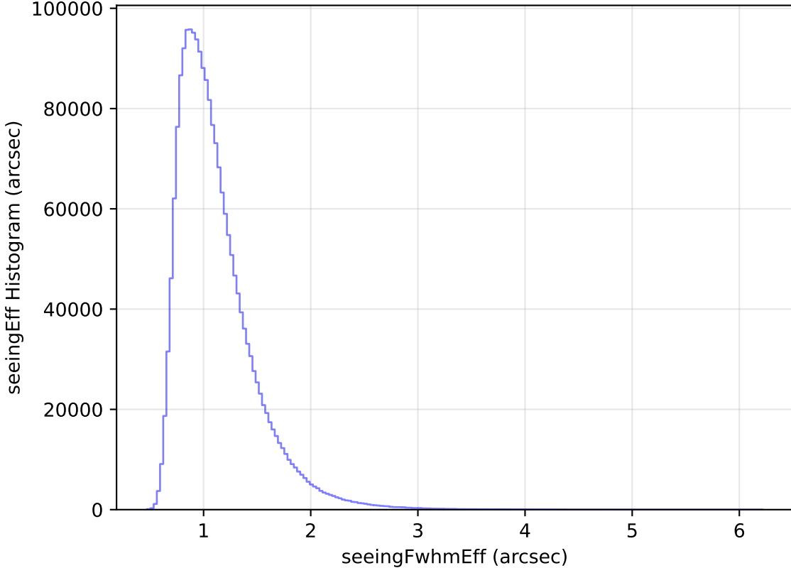
too_elab_heavy_r64_d2_griz_v3.4_10yrs WFD all bands: seeingEff Histogram
