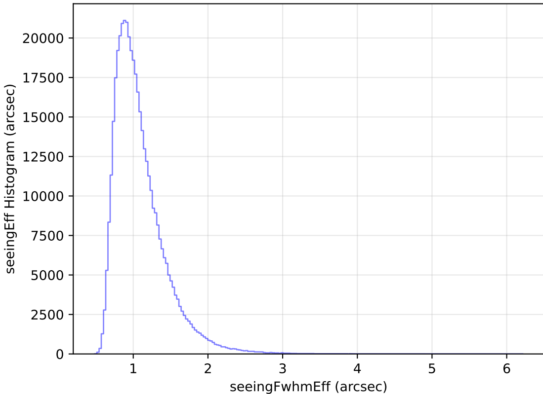
too_elab_heavy_r64_d2_griz_v3.4_10yrs All sky z band: seeingEff Histogram
