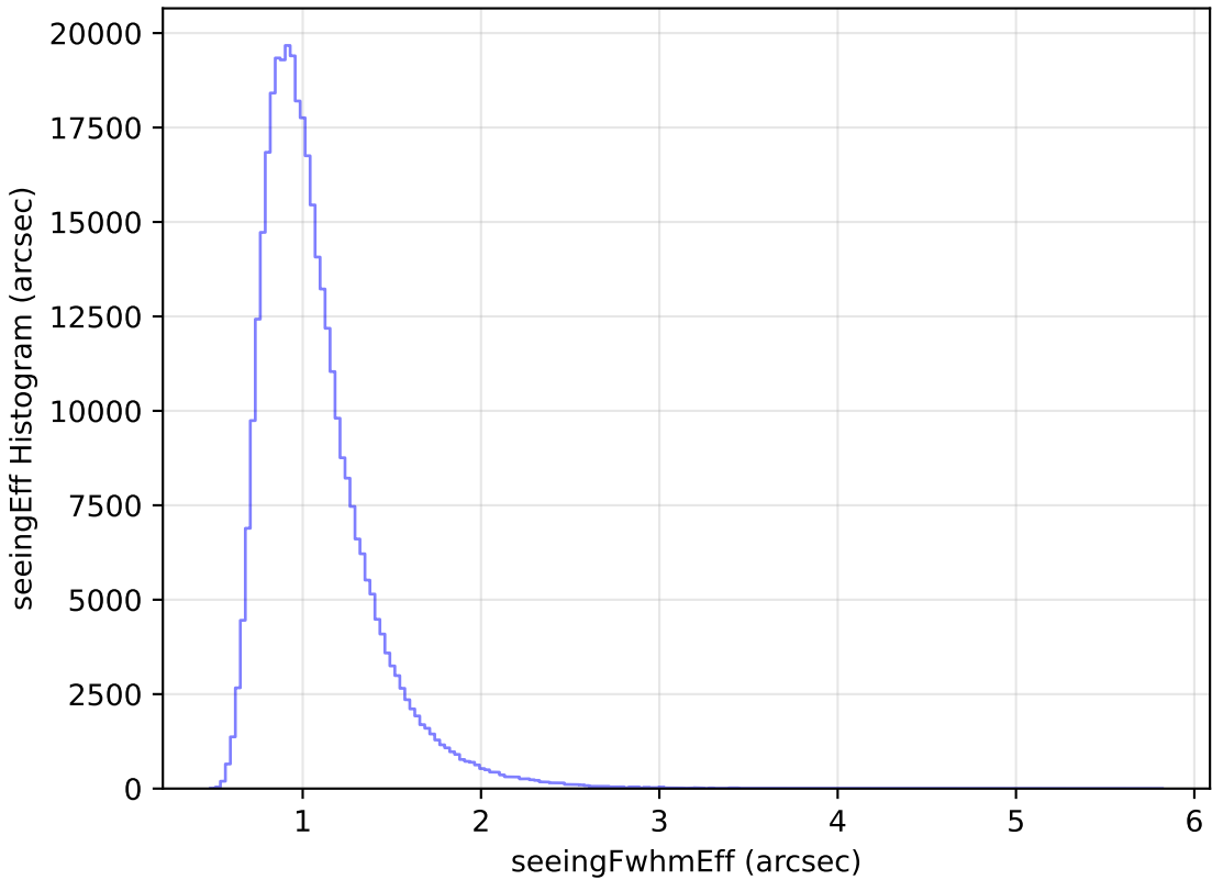
too_elab_heavy_r64_d2_griz_v3.4_10yrs All sky y band: seeingEff Histogram
