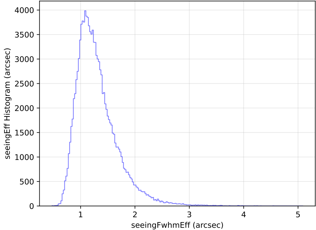
too_elab_heavy_r64_d2_griz_v3.4_10yrs All sky u band: seeingEff Histogram
