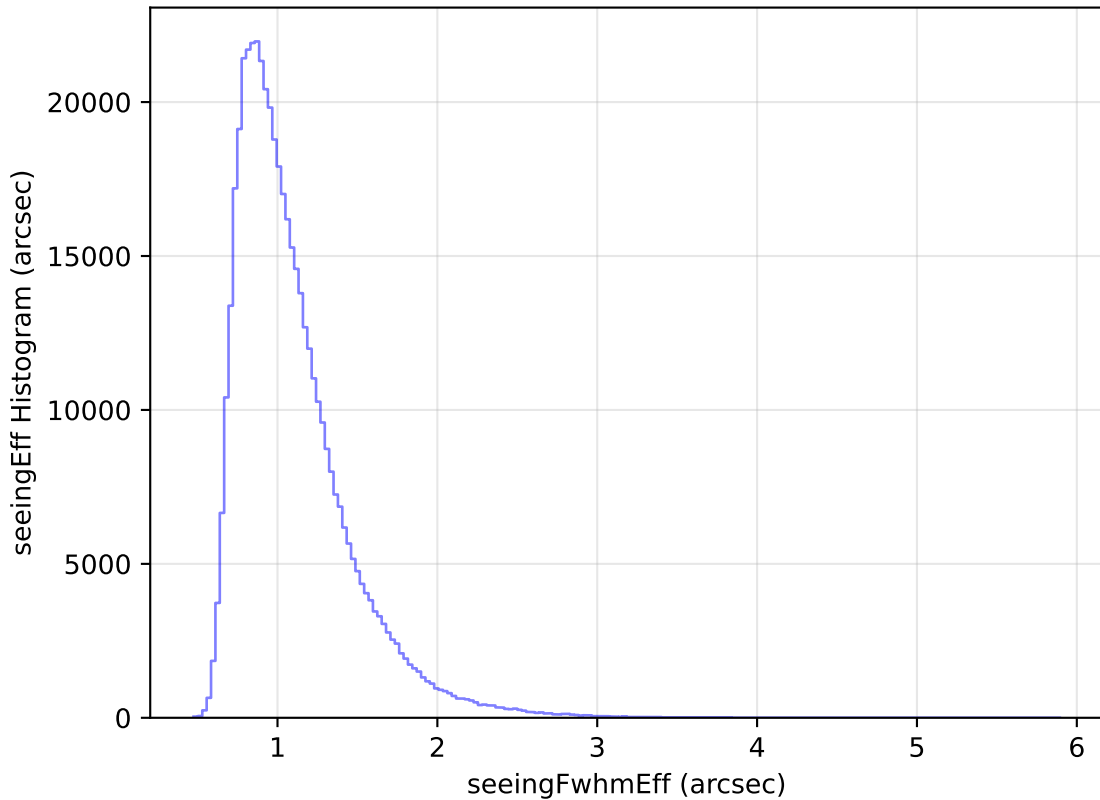
too_elab_heavy_r64_d2_griz_v3.4_10yrs All sky i band: seeingEff Histogram
