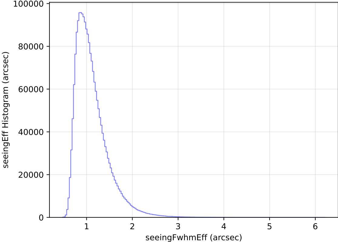
too_elab_heavy_r64_d2_griz_v3.4_10yrs All sky all bands: seeingEff Histogram
