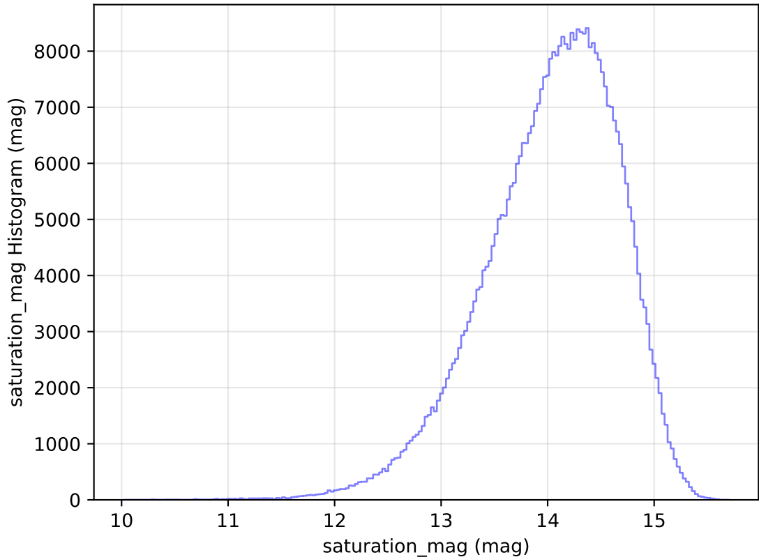
too_elab_heavy_r64_d2_griz_v3.4_10yrs WFD z band: saturation_mag Histogram
