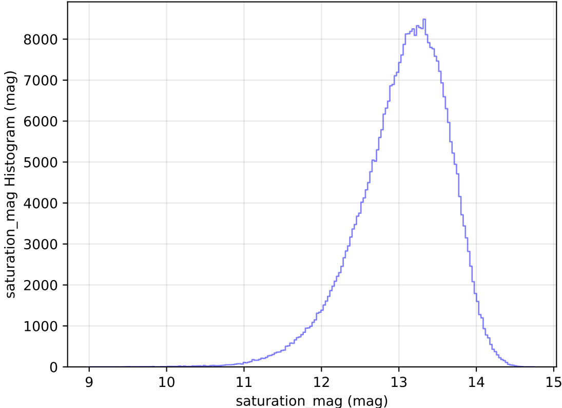
too_elab_heavy_r64_d2_griz_v3.4_10yrs WFD y band: saturation_mag Histogram
