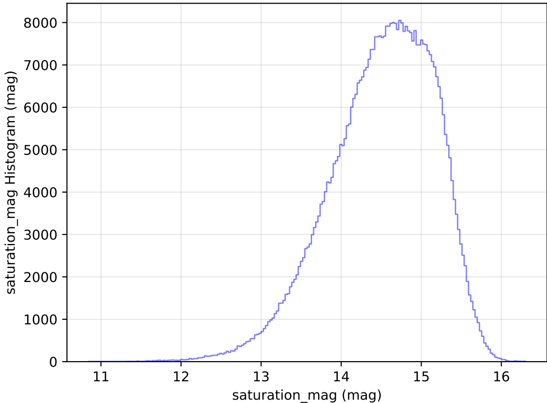
too_elab_heavy_r64_d2_griz_v3.4_10yrs WFD r band: saturation_mag Histogram
