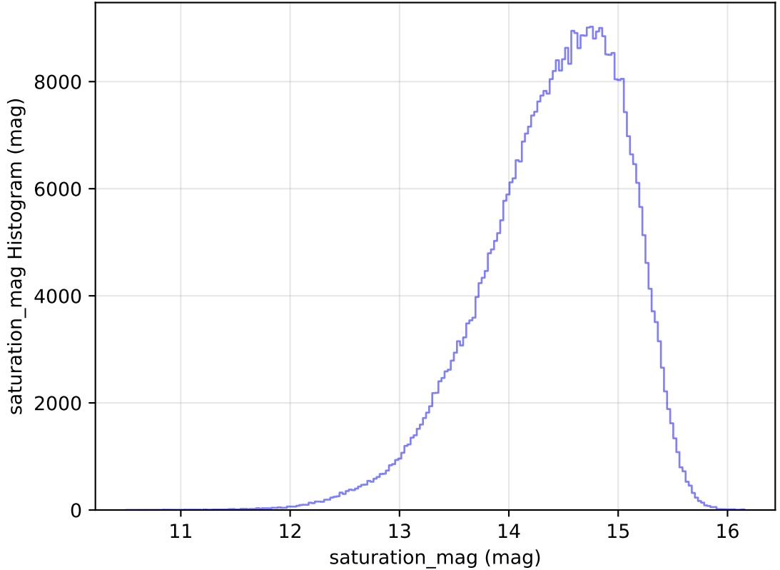
too_elab_heavy_r64_d2_griz_v3.4_10yrs WFD i band: saturation_mag Histogram
