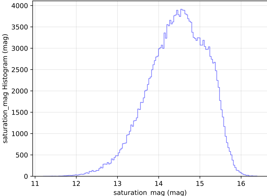
too_elab_heavy_r64_d2_griz_v3.4_10yrs WFD g band: saturation_mag Histogram
