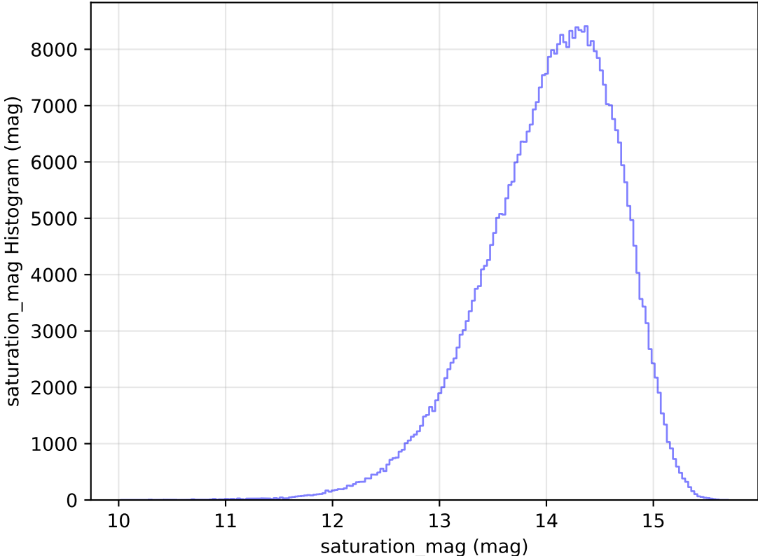
too_elab_heavy_r64_d2_griz_v3.4_10yrs All sky z band: saturation_mag Histogram
