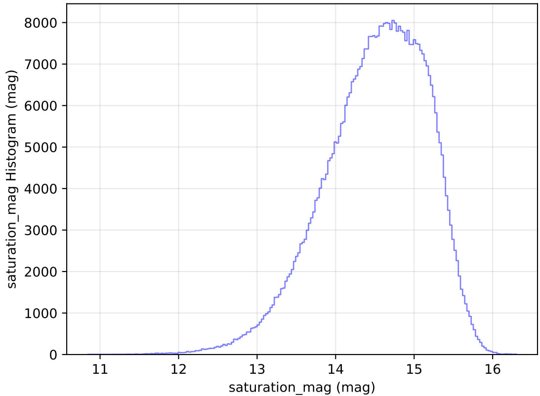
too_elab_heavy_r64_d2_griz_v3.4_10yrs All sky r band: saturation_mag Histogram
