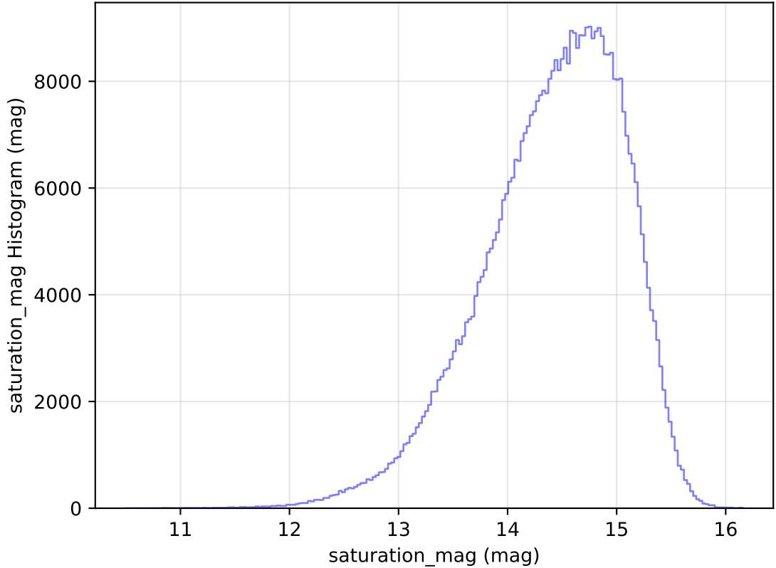
too_elab_heavy_r64_d2_griz_v3.4_10yrs All sky i band: saturation_mag Histogram
