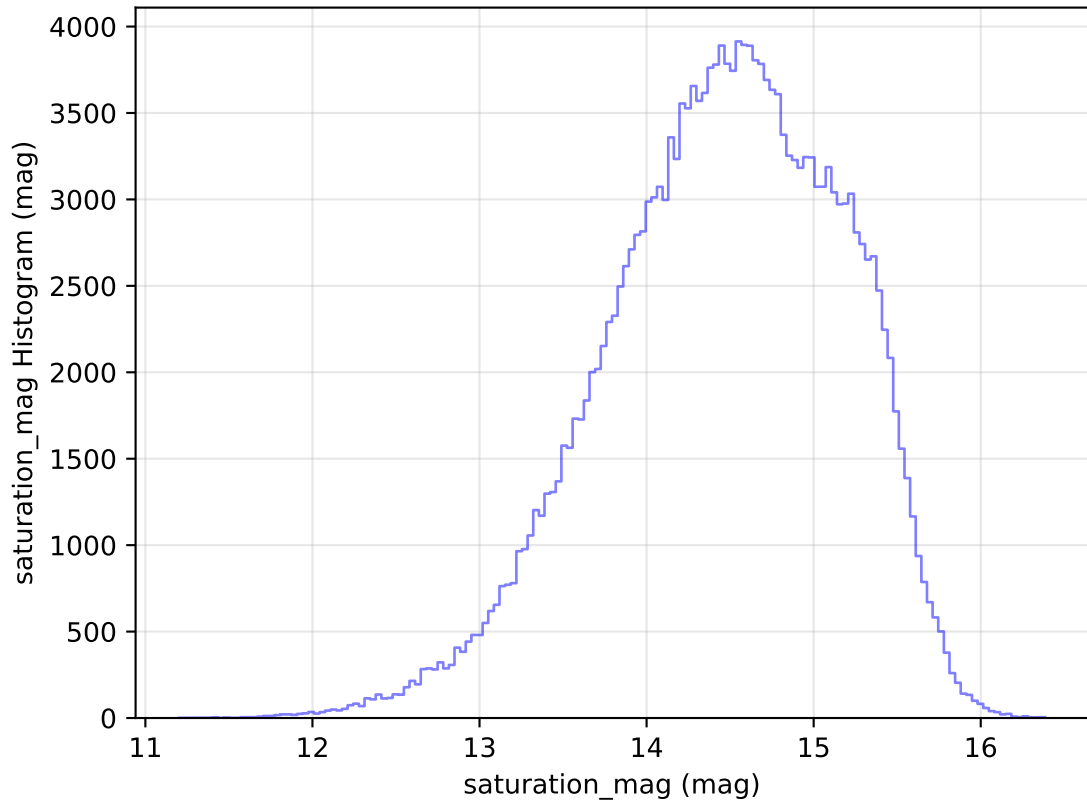
too_elab_heavy_r64_d2_griz_v3.4_10yrs All sky g band: saturation_mag Histogram
