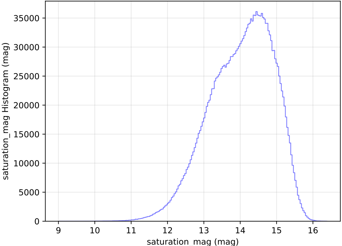
too_elab_heavy_r64_d2_griz_v3.4_10yrs All sky all bands: saturation_mag Histogram
