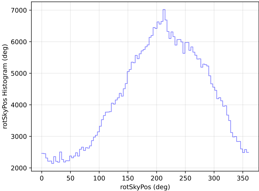
too_elab_heavy_r64_d2_griz_v3.4_10yrs WFD z band: rotSkyPos Histogram
