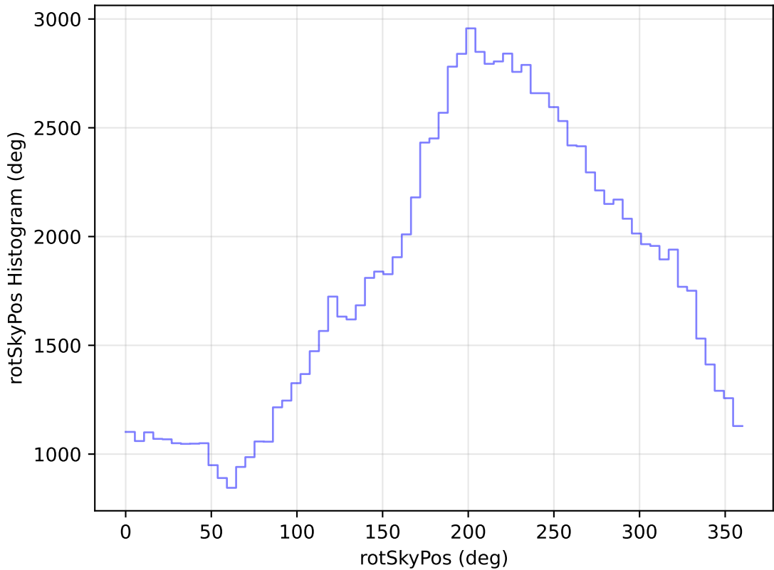
too_elab_heavy_r64_d2_griz_v3.4_10yrs WFD u band: rotSkyPos Histogram
