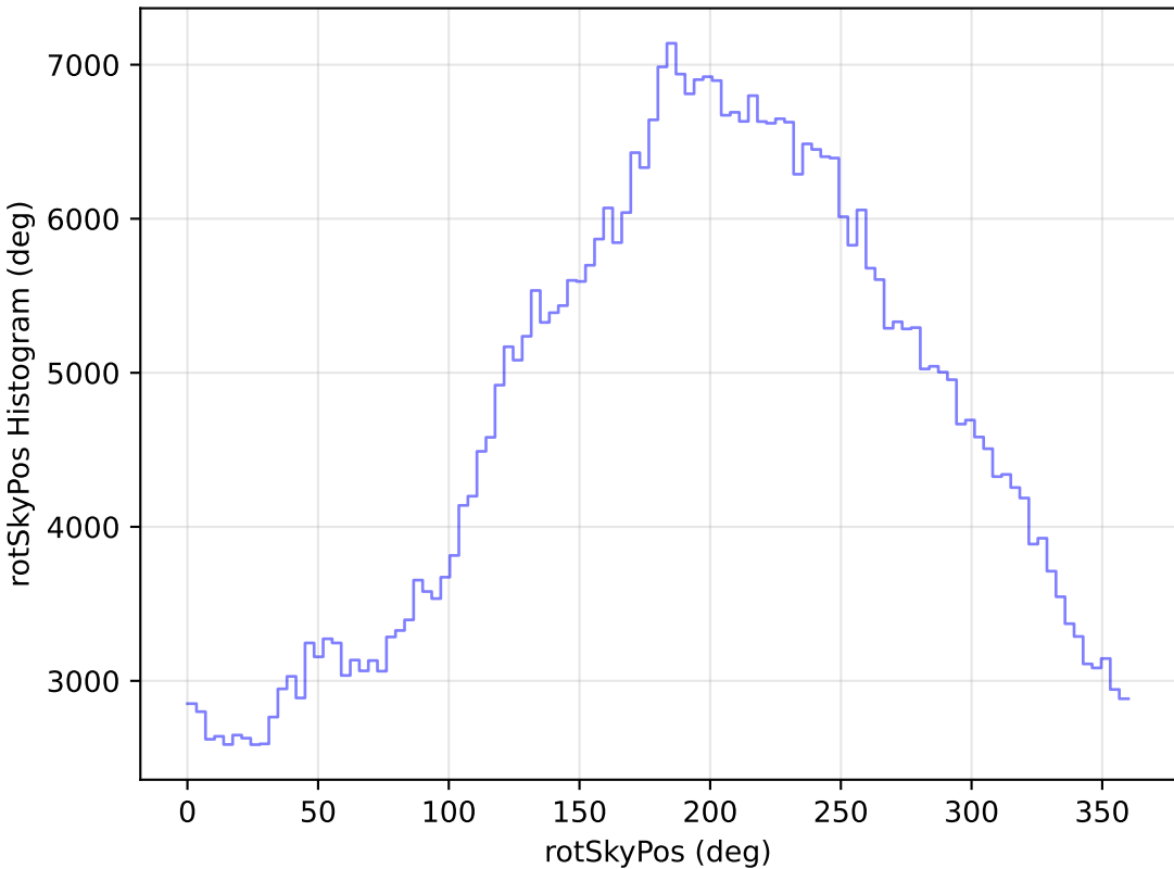
too_elab_heavy_r64_d2_griz_v3.4_10yrs WFD r band: rotSkyPos Histogram
