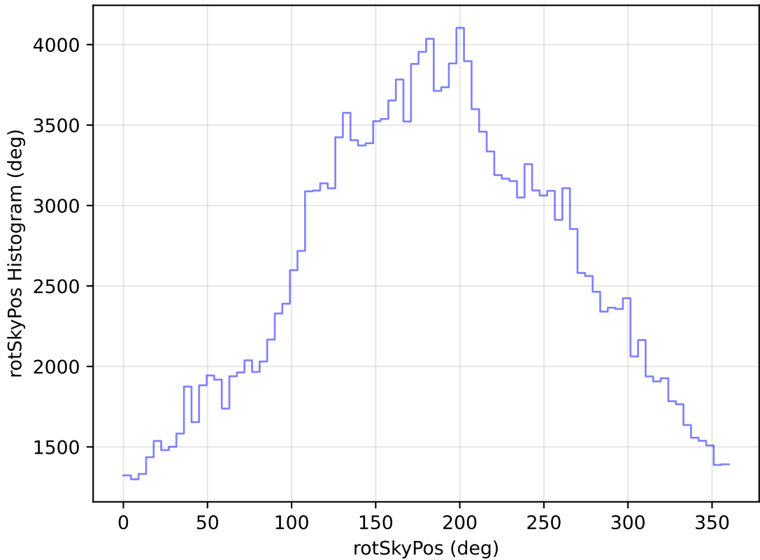
too_elab_heavy_r64_d2_griz_v3.4_10yrs WFD g band: rotSkyPos Histogram
