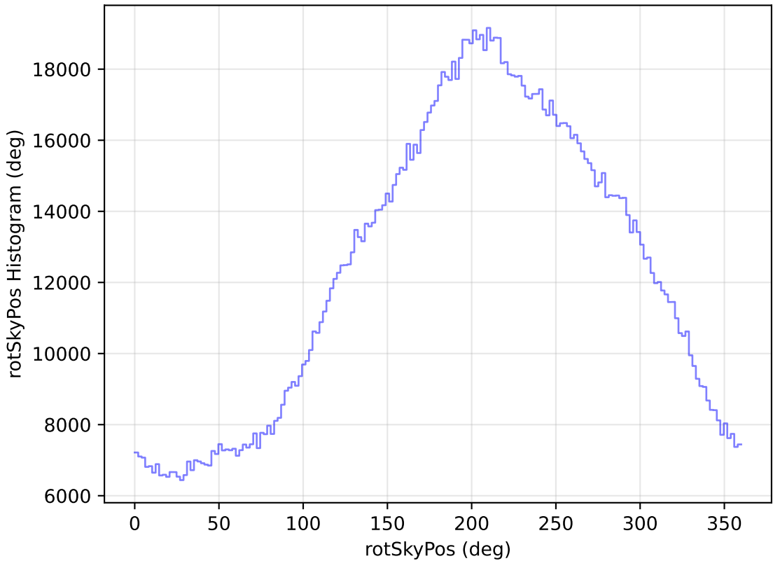
too_elab_heavy_r64_d2_griz_v3.4_10yrs WFD all bands: rotSkyPos Histogram
