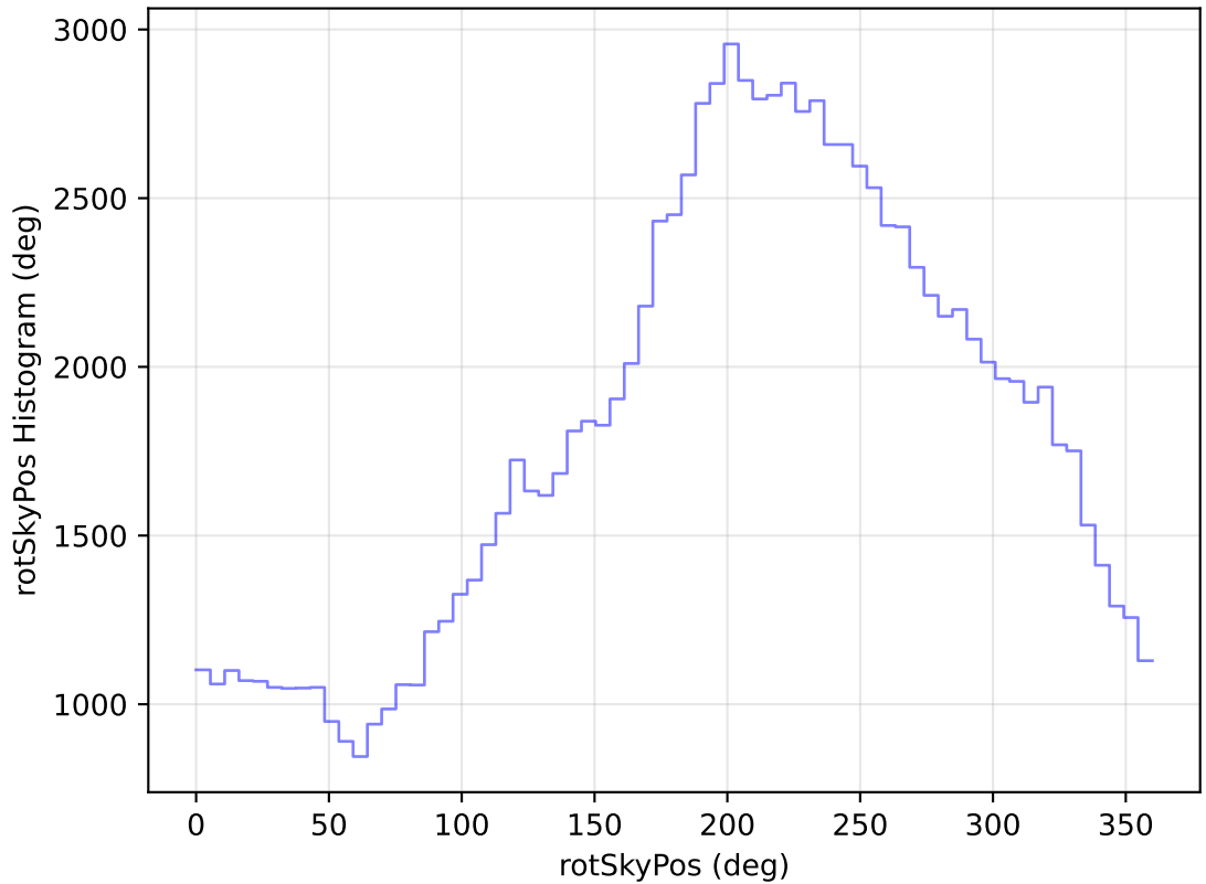
too_elab_heavy_r64_d2_griz_v3.4_10yrs All sky u band: rotSkyPos Histogram
