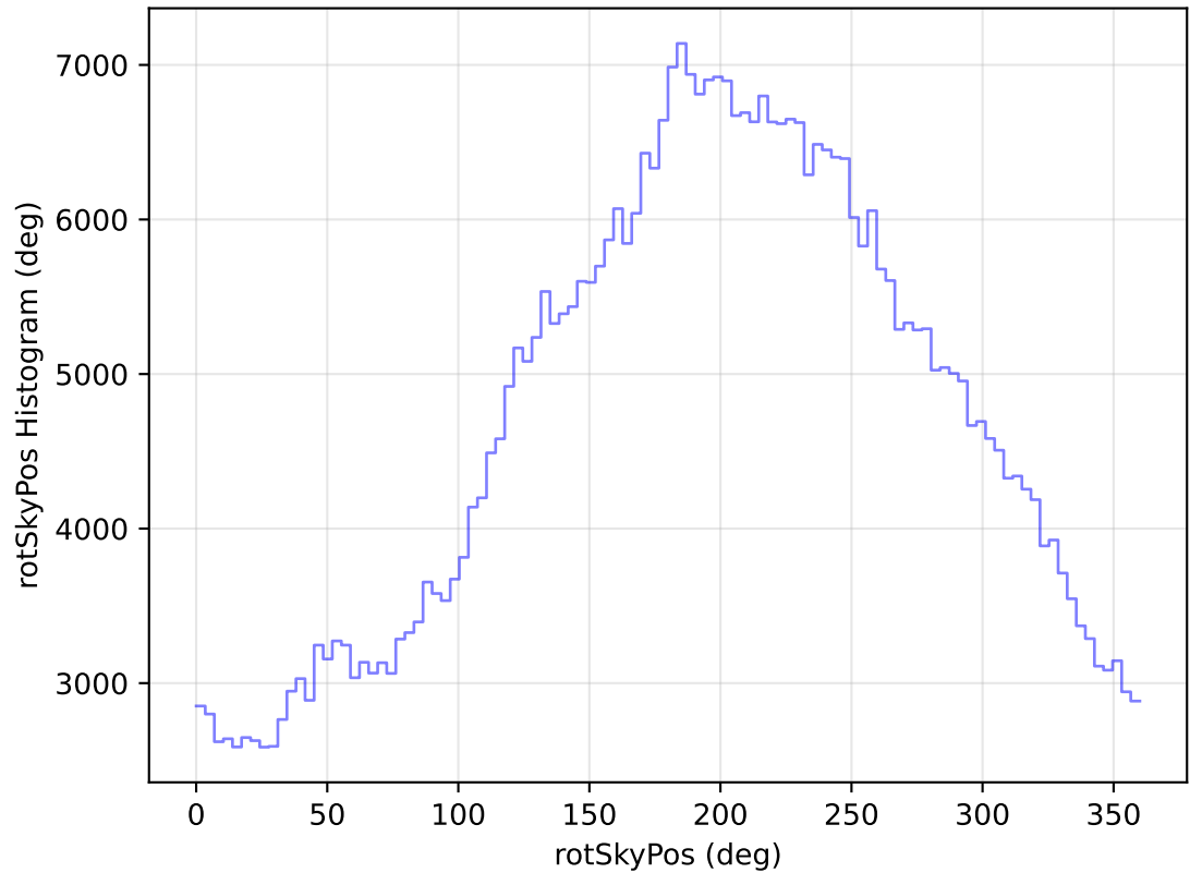
too_elab_heavy_r64_d2_griz_v3.4_10yrs All sky r band: rotSkyPos Histogram
