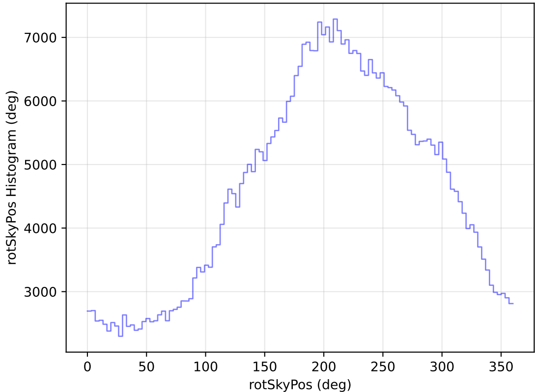
too_elab_heavy_r64_d2_griz_v3.4_10yrs All sky i band: rotSkyPos Histogram
